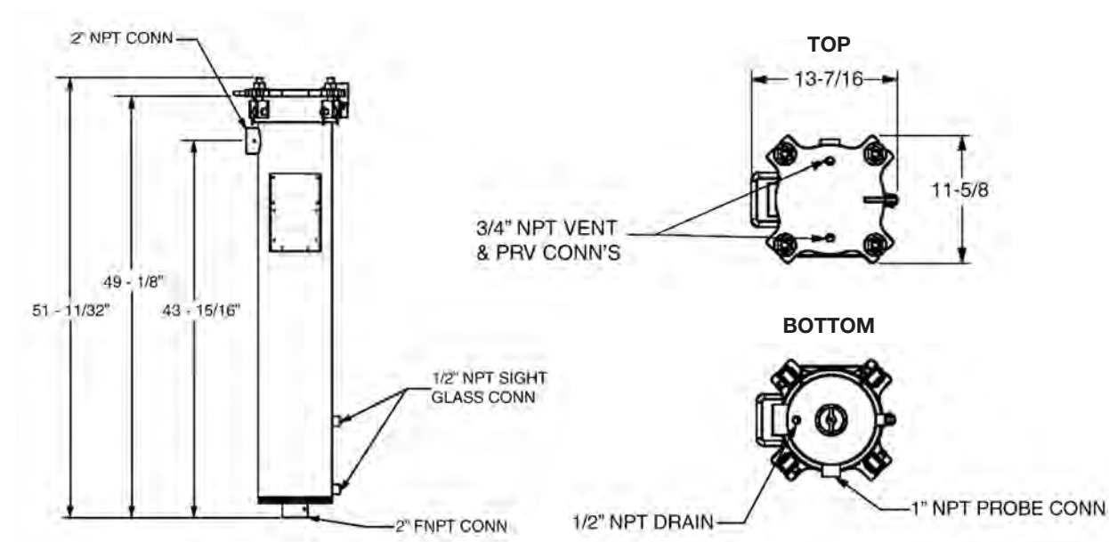
Drawing Shows Dimensions for VX-2
